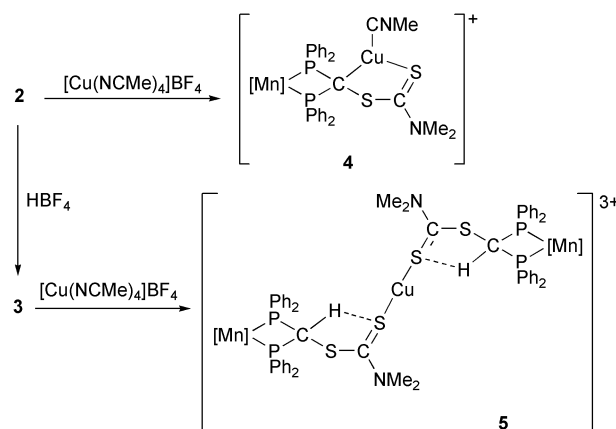
Scheme 2 Synthesis of complexes 4 and 5 . [Mn] = \text{Mn}(\text{CO})_4 .
