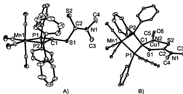
Fig. 1 ORTEP drawing of 2 (A) and 4 (B); hydrogen atoms are omitted for clarity. Selected bond distances [Å] and angles [°]: 2 : P(1)–C(1) 1.740(4), P(2)–C(1) 1.749(4), C(1)–S(1) 1.740(3), S(1)–C(2) 1.804(3), C(2)–S(2) 1.650(3), C(2)–N(1) 1.322(4); P(1)–C(1)–P(2) 100.79(17), C(1)–S(1)–C(2) 110.02(16). 4 : P(1)–C(1) 1.799(3), P(2)–C(1) 1.806(3), C(1)–S(1) 1.766(3), S(1)–C(2) 1.785(4), C(2)–S(2) 1.690(4), C(2)–N(1) 1.326(4), C(1)–Cu(1) 2.095(3), S(2)–Cu(1) 2.2317(9); P(1)–C(1)–P(2) 97.45(15), C(1)–S(1)–C(2) 108.91(16), C(1)–Cu(1)–S(2) 98.78, C(1)–Cu(1)–N(2) 138.91(12), S(2)–Cu(1)–N(2) 122.0(9).
