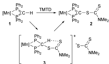
Scheme 1 Synthesis of complex 2 . [Mn] = \text{Mn}(\text{CO})_4 .
